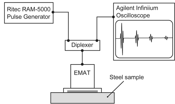
Figure 2. Shear wave measurement set-up
