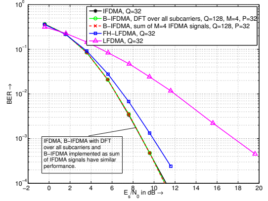
Fig. 3. Simulation of BER versus E_s/N_0 for the considered multiple access schemes. M =number of subcarriers per B-IFDMA block, P =number of blocks per chunk time with block size 4 subcarriers \times 3 OFDM symbols, and Q =number of subcarriers used in IFDMA, LFDMA and FH-LFDMA.
